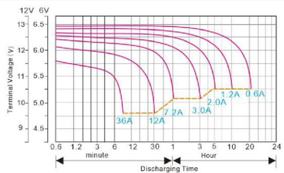
Discharge Characteristic (25°C/77°F)
